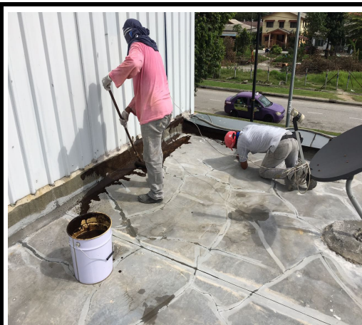
Photo 3 Apply primer bitumen at roof
