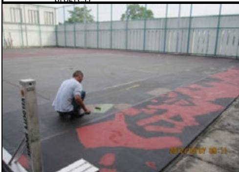
Photo 4 Patching mix. concrete and sand in progress
