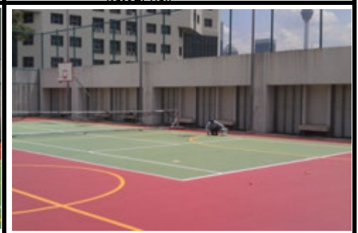
Photo 12 Another view of 4th coat of finish acrylic textured of green color in progress
