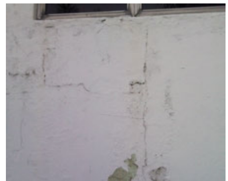
Photo 6 Defective plaster wall at side elevation near toilet area
